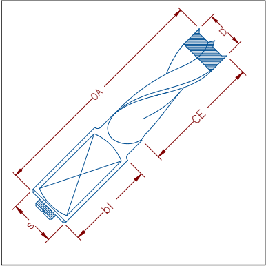
PD100 = 10mm x 20mm shank - 57mm over all length
