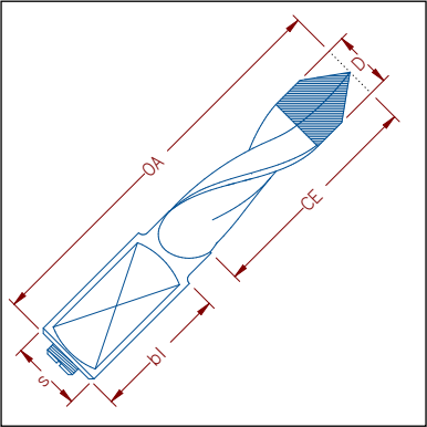
PD145 = 10mm x 20mm Shank - 57mm over all length
